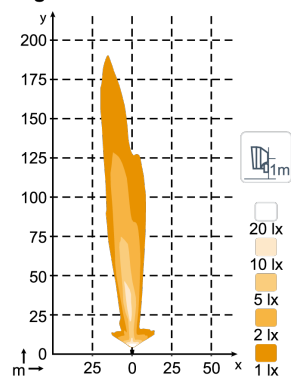
N5XX ECE High Beam
