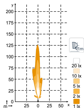
N5XX ECE Low Beam
