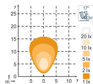
KL1305 800lm Wide Flood
