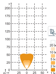
N4405 QD, N4406 2100lm Low Beam
