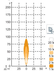
N26 700lm Flood
