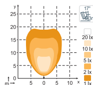
N4405 QD, N4406 2100lm Wide Flood
