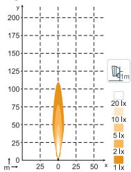
N2401 600lm Diffused
