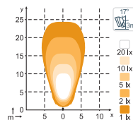
N4409 QD, N4410 2000lm Flood
