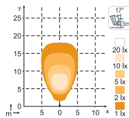
N2401 750lm Flood
