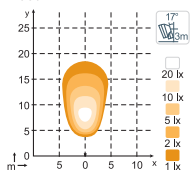
KL1305 800lm Flood
