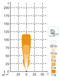
N31 2100lm High Beam
