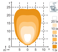
N4401 QD, N4402 4200lm Wide Flood
