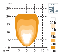
N4409 QD, N4410 2000lm Wide Flood
