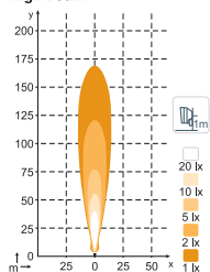
N4409 QD, N4410 2000lm High Beam
