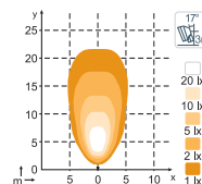
N4405 QD, N4406 2100lm Flood
