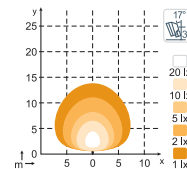
N4405 QD, N4406 1680lm Diffused
