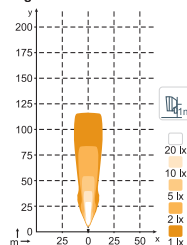
N4405 QD, N4406 2100lm High Beam
