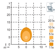
KL1501 300lm Flood
