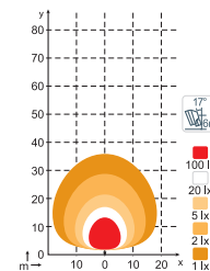
N4702 14400lm Diffused
